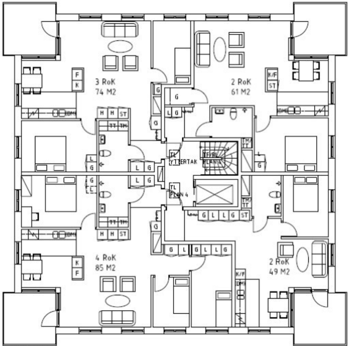
PLAN 3-4
