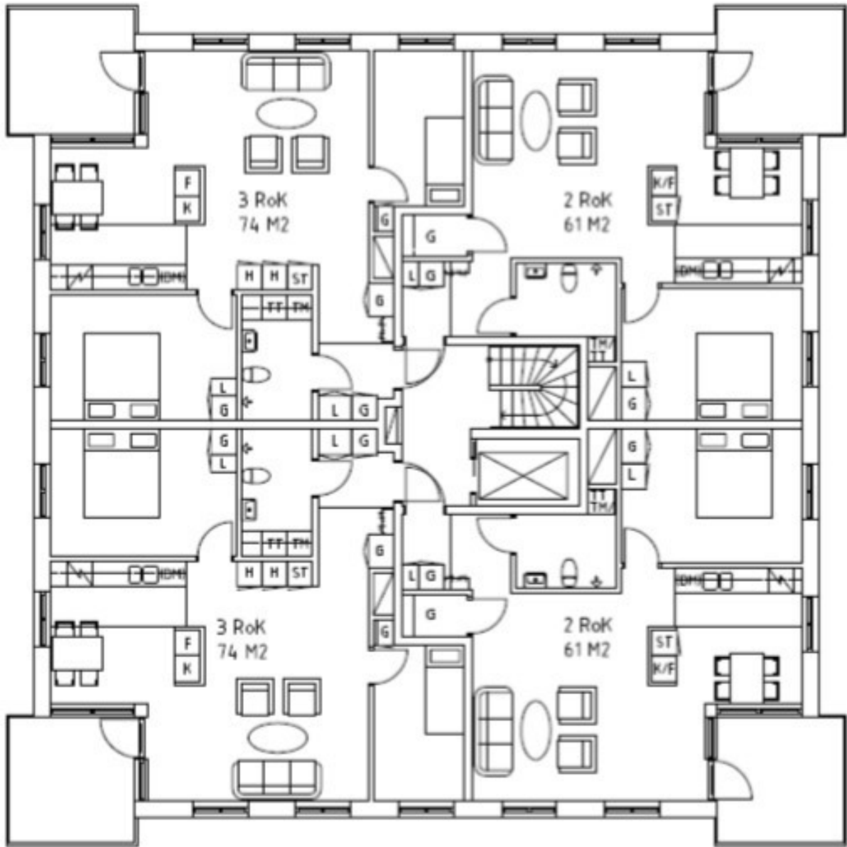
PLAN 2
